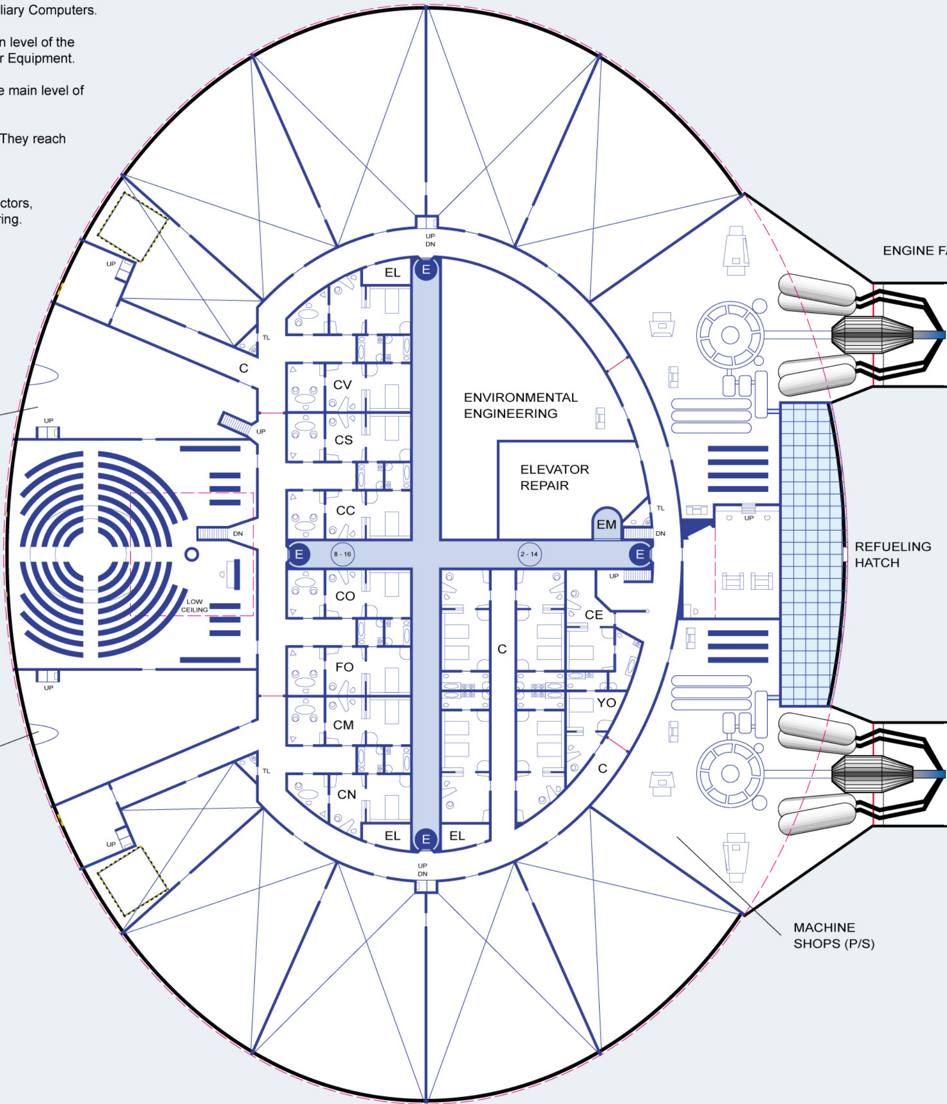
DECK 10: CARGO / OFFICERS' QUARTERS / ENGINEERING
